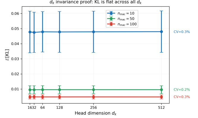
Fig. 2. \mathbb{E}[\text{KL}] vs. d_k \in \{16, 32, 64, 128, 256, 512\} for n_{\text{mac}} \in \{10, 50, 100\} , n_{\text{seq}} = 64 . CV \leq 2\% across all d_k ; one-way ANOVA p = 0.90 , confirming Theorem 3.
