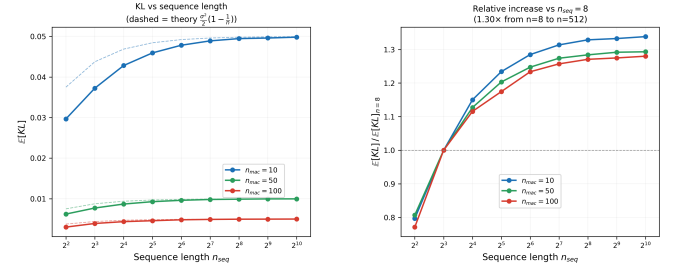
Fig. 3. Left: \mathbb{E}[\text{KL}] vs. n_{\text{seq}} for n_{\text{mac}} \in \{10, 50, 100\} (solid) and theory (1/(2n_{\text{mac}}))(1 - 1/n_{\text{seq}}) (dashed). Right: KL ratio relative to n_{\text{seq}} = 8 ; a 64\times increase in n_{\text{seq}} raises KL by only 1.30\times .
